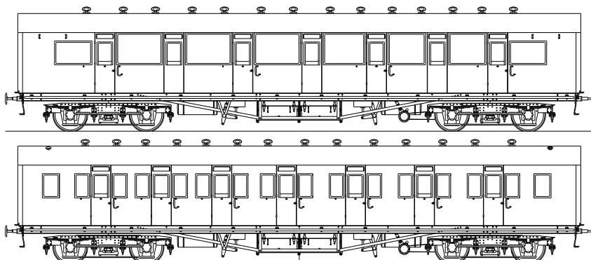
7C026 Seven Compartment Composite (Diagram 2301)
