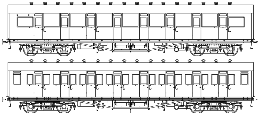
7C024 Eight Compartment All Third (Diagram 2001)
