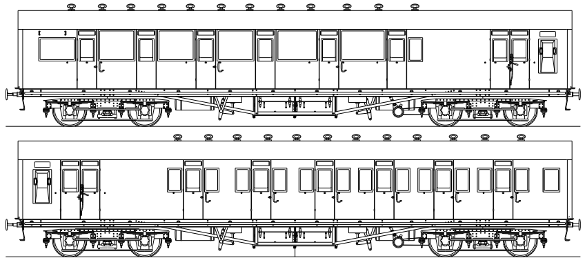
7C023 Six Compartment Brake Composite (Diagram 2401)
